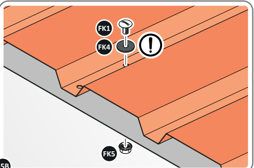
35B SECURE ROOF PANELS AT x8 LOCATIONS INDICATED USING TYPICAL FIXING METHOD. IMPORTANT: ENSURE RUBBER WASHER FK4 IS LOCATED AS SHOWN.
