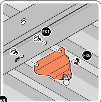
50C ALIGN EACH GAS STRUT BRACKET WITH RELEVANT FIXING ANGLES, SECURE USING TYPICAL FIXING METHOD ABOVE.
