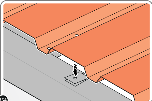
35A LOCATE A ROOF PANEL SIDE 0212-05 ALIGN WITH AIR BEND TABS AS INDICATED.
