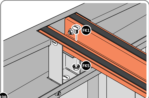
33B SECURE ROOF CHANNEL ASSEMBLY AT EACH FIXING POINT (x3 EACH SIDE) USING FASTENERS DETAILED ABOVE.
