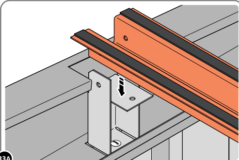
33A SLOT EACH ROOF CHANNEL ASSEMBLY 0215-06 INTO ROOF SUPPORT.
