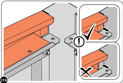
LOCATE ROOF SIDE INFILL 0212-12 AS SHOWN ABOVE.
