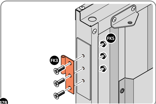
47B SECURE DOOR HINGE PLATE AND HINGE 0203-27 AND 0203-28 AS SHOWN. IMPORTANT: ENSURE CORRECT DOOR HINGE IS SECURED TO CORRECT DOOR.
