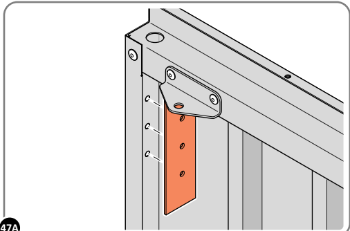
47A LOCATE DOOR HINGE PLATE 0203-37 WITHIN DOOR AS SHOWN.
