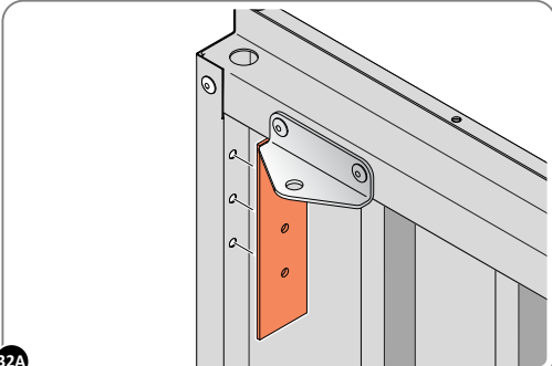
32A LOCATE DOOR HINGE PLATE 0203-37 WITHIN DOOR AS SHOWN.
