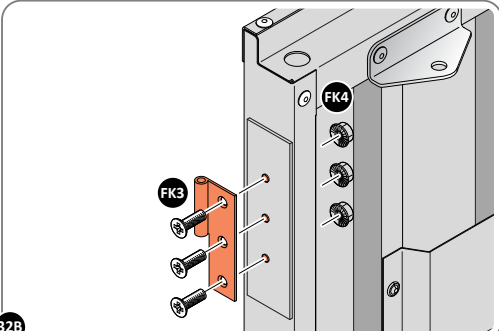
32B SECURE DOOR HINGE PLATE AND HINGE 0203-27 AND 0203-28 AS SHOWN. IMPORTANT: ENSURE CORRECT DOOR HINGE IS SECURED TO CORRECT DOOR.
